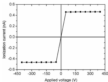
Figure 3. Saturation curve of the ionization chamber. The maximum uncertainty was 0.1%, and is therefore not visible in the figure.
