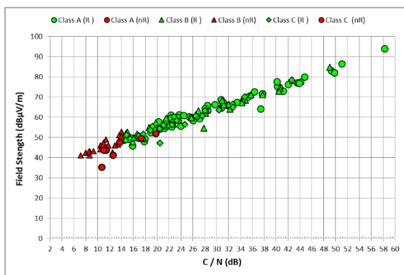
Figure 4. Field strength vs C/N (silicon tuner)
