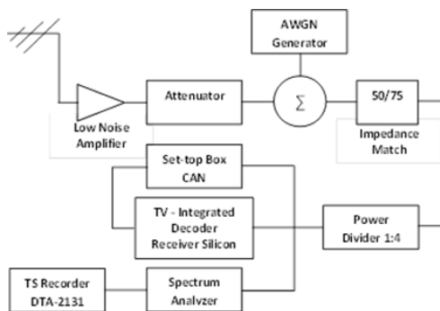
Figure 1. Reception setup.
