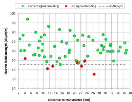
Figure 3. Field strength vs. distance (silicon tuner)
