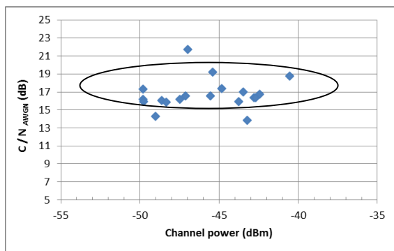
Figure 5. C/N_{awgn} achieved from field tests
